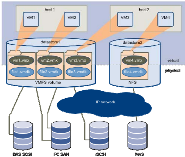
Figure 3: Storage Virtualization
